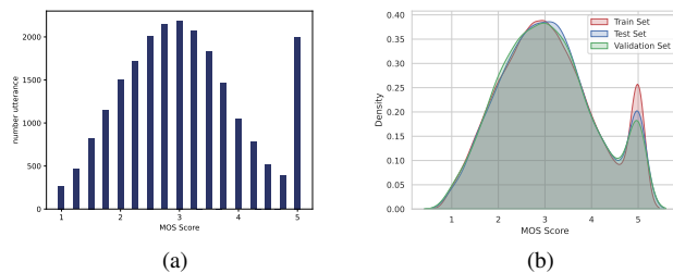
Fig. 4. (a) The MOS score distribution of the VCC2018-CSMSC dataset. The horizontal axis represents the MOS values, while the vertical axis represents the number of audio samples corresponding to each MOS value; (b) KDE diagram of the train, valid, and test set using the hold-out splitting method. The horizontal axis represents the MOS values, while the vertical axis represents the density corresponding to each MOS value.
